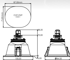
PE01 SPOT LIGHT 87x71 mm 4 W
