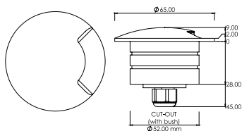
L9809 COURTESY LIGHT Ø mm 65 1 W
