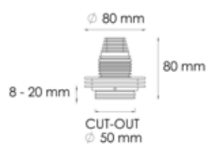
L3500 COURTESY LIGHT \varnothing mm 50 6 W
