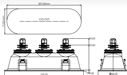
PE03 SPOT LIGHT 207x71 mm 3x4 W
