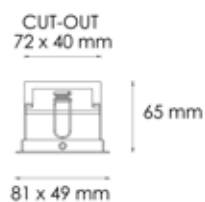
L4202 FIXED RECESSED LUMINAIRES mm 81x49 2x4 W
