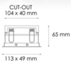
L4203 FIXED RECESSED LUMINAIRES mm 113x49 3x4 W
