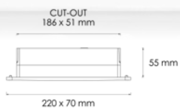
L9007 FLOODLIGHTS mm 220x70 36 W
