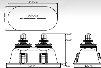
PE02 SPOT LIGHT 147x71 mm 2x4 W
