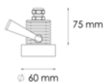
L0163 SPOTLIGHT Ø mm 60 4/6 W
