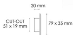
L0215 COURTESY LIGHT mm 35x79 1 W IP 40/65
