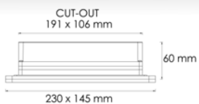
L9114 FLOODLIGHTS mm 230x145 36 W
