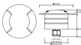
L9810 COURTESY LIGHT Ø mm 65 2x1 W
