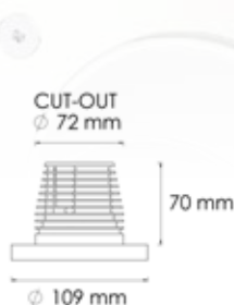
L0159 SPOTLIGHT Ø mm 109 11 W
