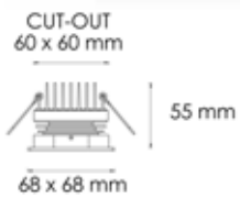
L8006 RECESSED LUMINAIRES 60x60 mm 6 W
