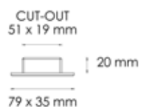
L0214 COURTESY LIGHT mm 79x35 1 W IP 40/65
