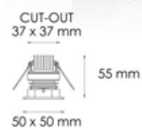
L8002 RECESSED LUMINAIRES 50x50 mm 6 W
